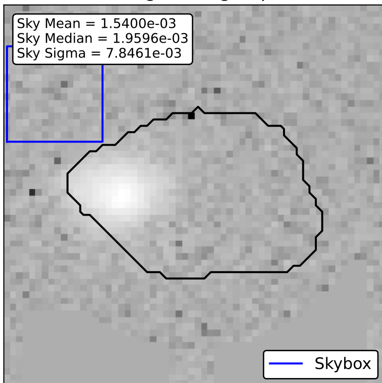
Original Segmap
