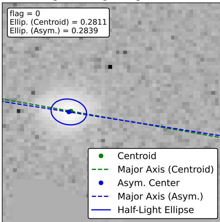
Original Segmap
